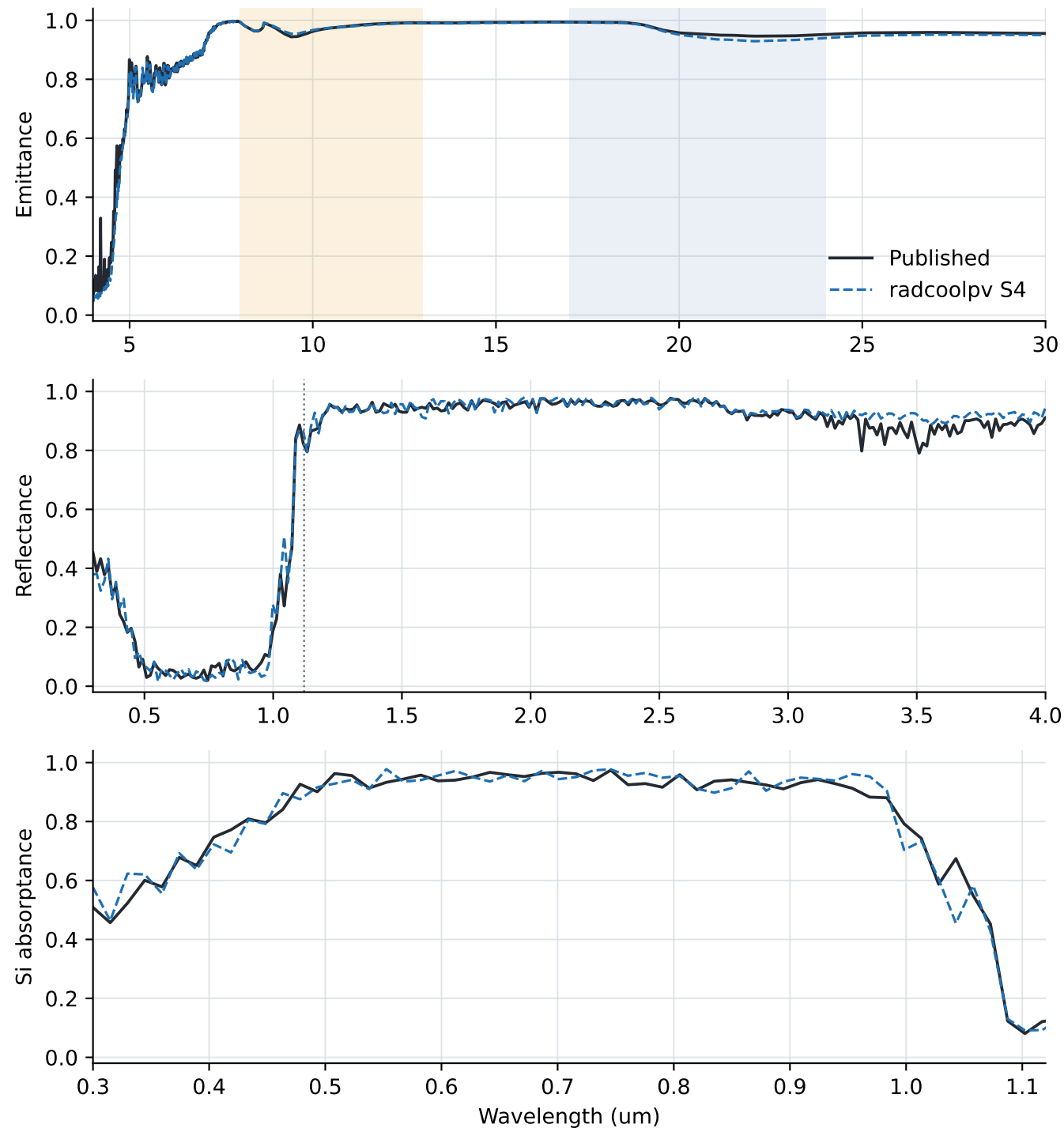
Validation A.1 normal-incidence spectral comparison
